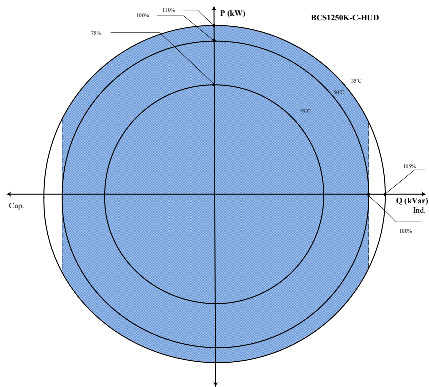
Rated grid voltage P-Q Curve(Different temperature)
